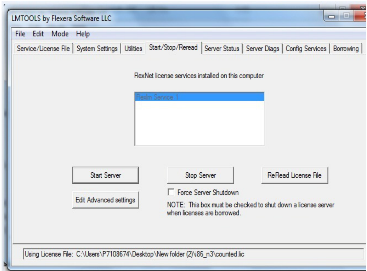
Figure 10-3: Start/Stop/Reread Tab
